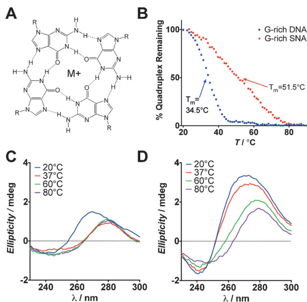
Figure 1. A) G-quartet structure stabilized by M^+ ( \text{Na}^+ , \text{K}^+ , etc.) B) CD spectroscopy was used to measure the melting temperature ( T_m ) of G-quadruplexes formed on the SNA and with linear G-rich DNA. The full CD spectra for C) G-rich DNA and D) G-rich SNAs are shown at increasing temperatures, demonstrating the enhanced thermal stability of G-quadruplexes formed on the SNA scaffold.
